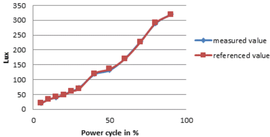
Fig. 10. Comparison of the measured value of LACFSOC lux against the referenced value of lux with different values of power cycle %
