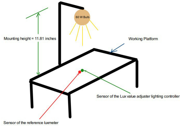
Fig. 8. Representational diagram of setup for corroboration
